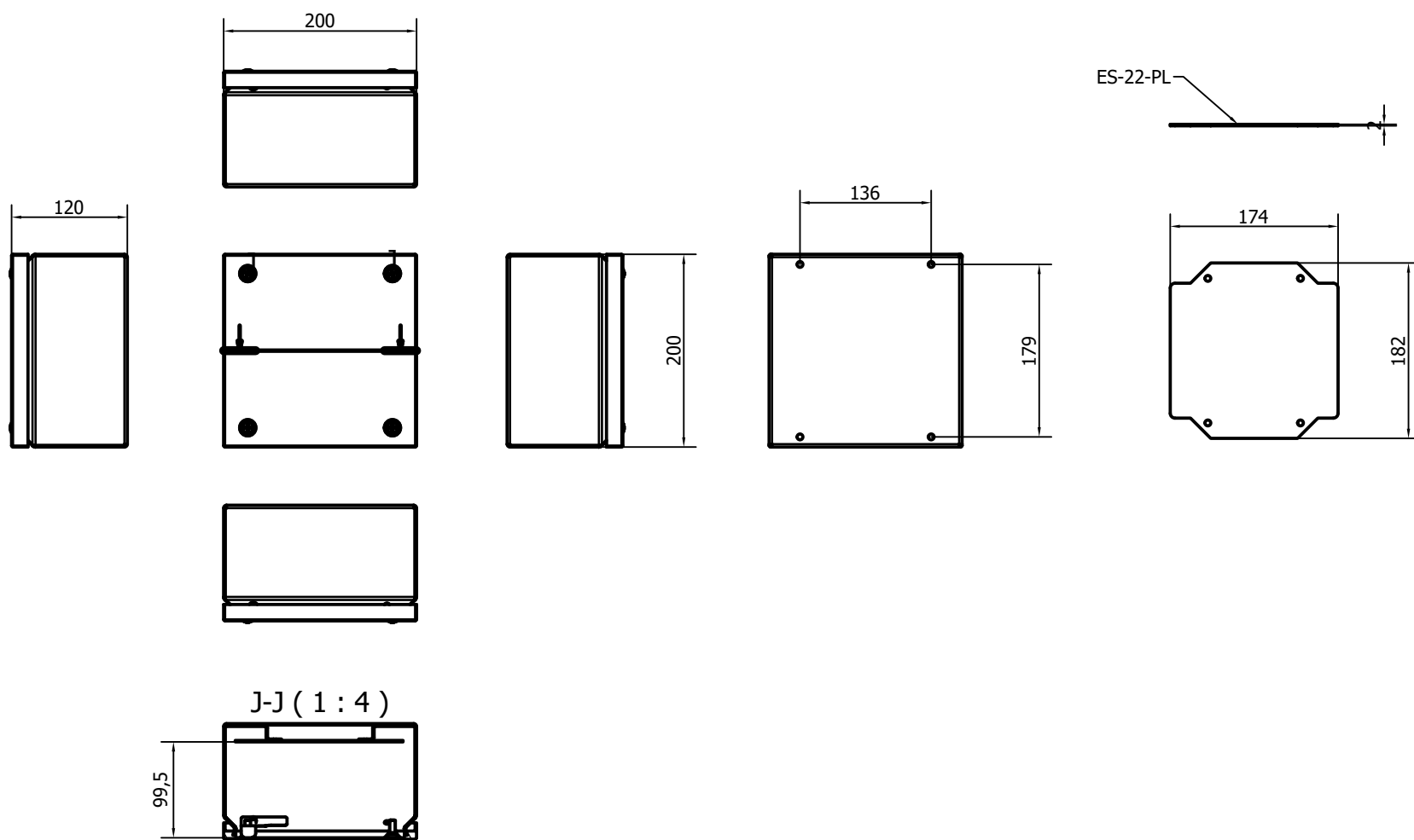
ES22 Junctions Box H200xL200xP120 RAL7035
